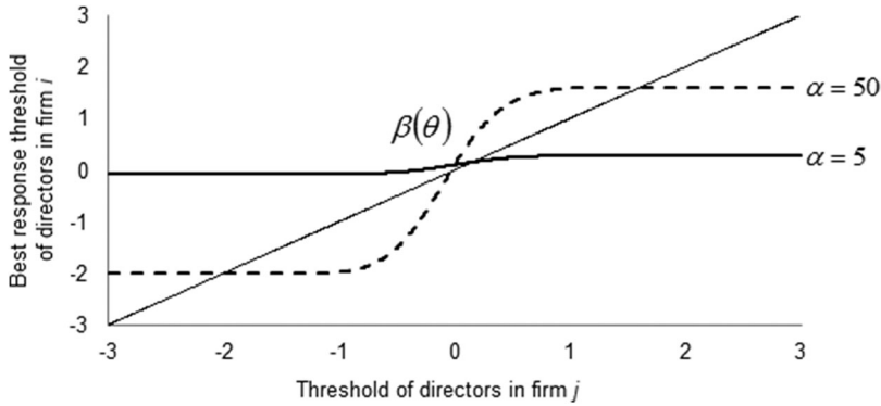
Figure 1. Best response function. The figure presents directors’ best response function \beta(\theta) for parameters \delta = 0.2, K = 9, T = 5, v(1, \theta) = e^{0.4\theta}, v(0, \theta) = e^{-0.2\theta} + e^{0.08} - e^{0.02} , and a standard normal distribution of types, where \delta is the probability that a firm is hit by a resignation shock, K is the number of directors on the board, T is the voting rule, and v(\cdot, \theta) is the utility of a director of type \theta from the allocation of control in his firm. Parameter \alpha measures the strength of directors’ reputational concerns.
