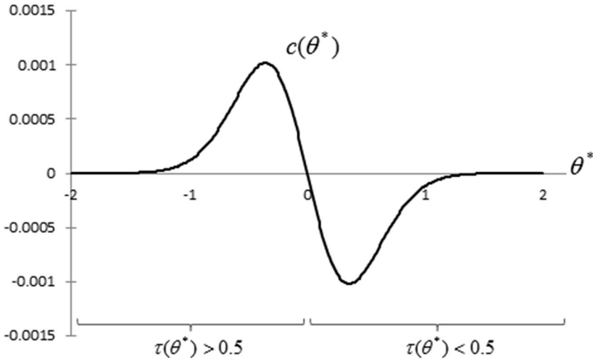
Figure 2. Board composition. The figure presents the average type of the board c(\theta^*) as a function of the equilibrium threshold \theta^* for parameters \delta = 0.2 , K = 9 , T = 5 , and a standard normal distribution of types, where \delta is the probability that a firm is hit by a resignation shock, K is the number of directors on the board, and T is the voting rule. \tau(\theta^*) is the equilibrium probability of shareholder control in a given firm.
